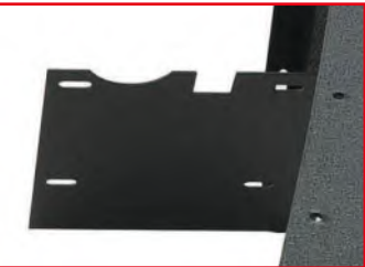
INTERNAL REINFORCEMENT
