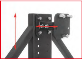
TWO WAY ADJUSTABLE TIRE MOUNT
